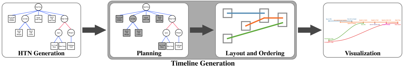
Figure 3: Overview of Yarn’s four stage pipeline: (1) generate Hierarchical Task Networks for each of the character entities in the narrative; (2) HTN planning to generate timelines; (3) compute the layout and ordering of the entities in each timeline; and (4) create visualizations inside a browser window
