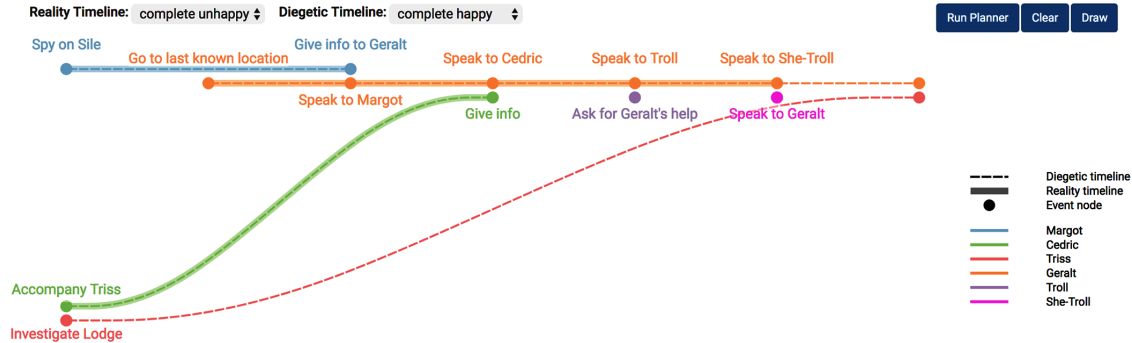
Figure 1: Yarn visualization depicting both actual (reality) and alternate (diegetic) narrative timelines. Colored lines trace the path of the main characters as a narrative progresses over time. Solid and dashed lines connect events on the reality and diegetic timelines, respectively. Nodes on the y-axis represent character sub-goals, and vertical node clusters represent events
