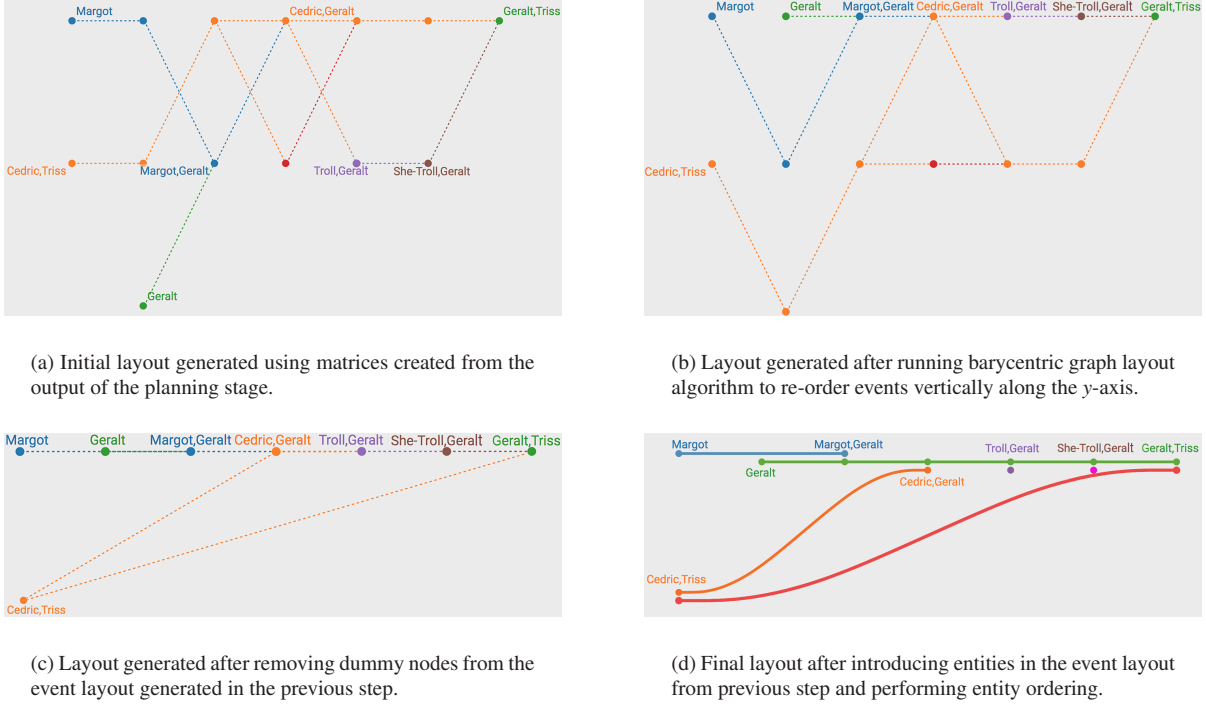
Figure 4: Illustration of various steps of the layout and ordering stage applied to a timeline for the example narrative in Sect. 5.1
