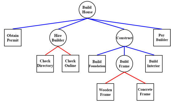
Figure 2: A hierarchical task network decomposing the task “Build House”. Rectangular nodes represent primitive actions, and circular nodes represent (sub-)tasks in the decomposition. Red lines show decomposition for an OR node, while blue lines show decomposition for an AND node
