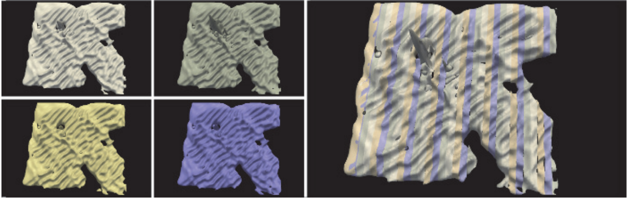
Figure 7. Weather Fire Burn Simulation Side-by-side vs. ESS: 4 potential temperature surfaces where t \in [287^\circ\text{F}, 345^\circ\text{F}] . The bottom two surfaces in the left quad are almost identical; the other two surfaces (top row of quad), are the most different in the set. The ESS visualization (right image) shows both similarities as well as high/low frequency differences between all surfaces in the ensemble. The large differences near the peak in the upper part of the images are visible in side-by-side visualization, but the subtle changes in location of the features in the lower right is difficult to see. Dark gaps between sets rapidly draw attention to both differences in the ESS view.
